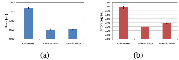
Fig. 4. Overall localization error in simulation. (a) Position error. (b) Heading error. Error bars denote 95% confidence intervals.
