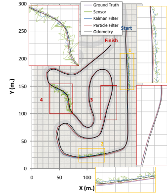
Fig. 3. Localization results in simulation.
