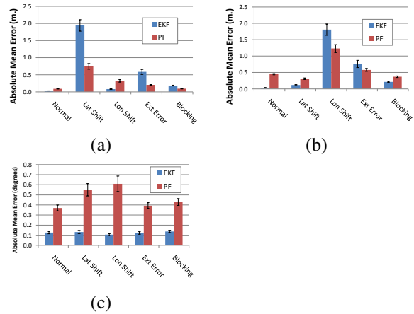
Fig. 11. Evaluation of our proposed method compared to EKF-based localization. (a) Lateral error. (b) Longitudinal error. (c) Heading error.
