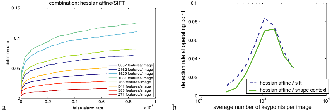
Figure 12. Panel a: ROCs obtained when varying the threshold T_{\text{det}} on minimum saliency that a region has to satisfy in order to be declared a feature. The legend shows the average number of features detected per image. The chosen operating point is displayed by a vertical line. ROCs are displayed for the hessian-affine/SIFT combination. Panel b is another representation of the data from panel a taken at the operating point. Here the horizontal axis is the average number of features per image, which was displayed in the legend in panel a. Results are displayed for the two combinations that performed best in Section 6.1, while panel a shows results only for one combination.
