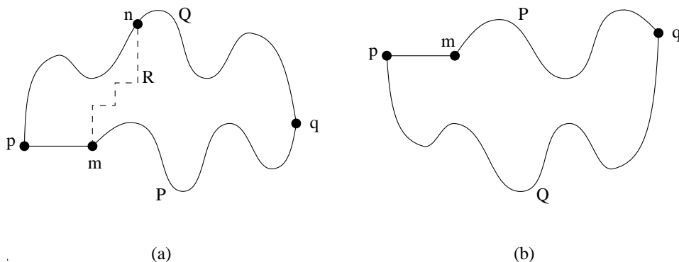
Figure 2: Illustration for the proof of Proposition 2.
