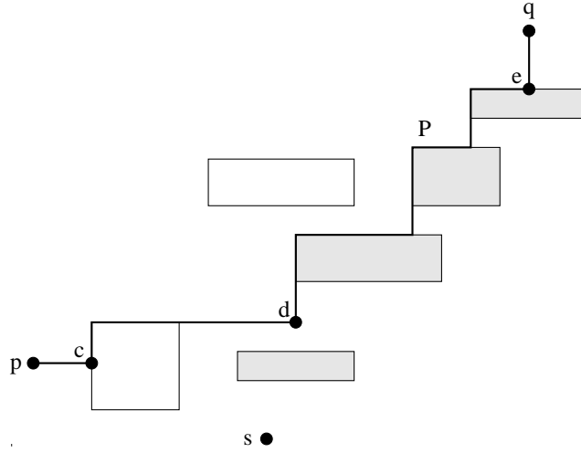
Figure 1: The shaded rectangles comprise a horizontal blockage between s and q ; P is the x -first path from p to q .
