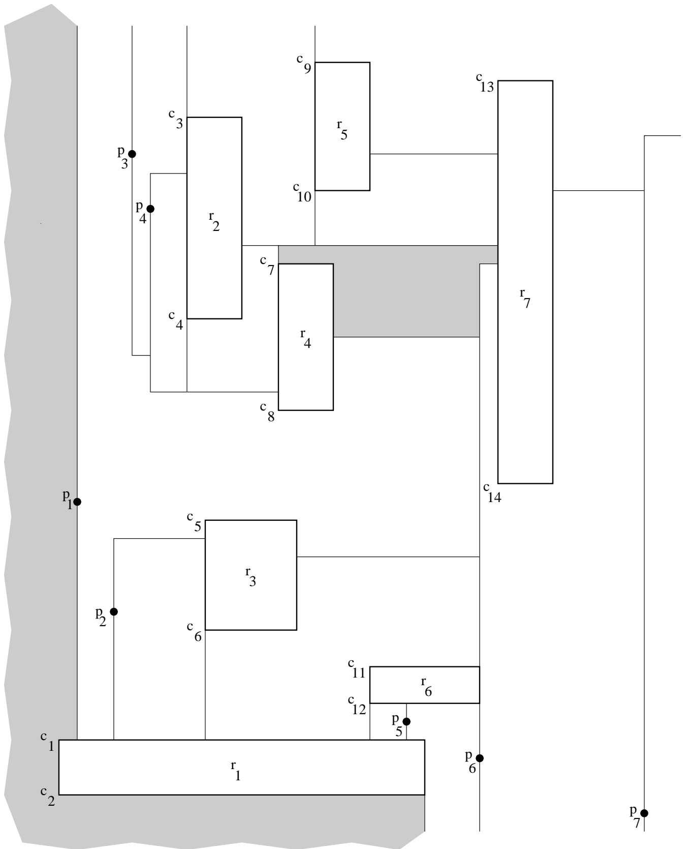
Figure 9: The x -diagram X_R(S_1) , for S_1 = \{p_1, p_2, p_3, p_4, p_5, p_6, p_7\} and R = \{r_1, r_2, r_3, r_4, r_5, r_6, r_7\} . The shaded region on the left consists of points that cannot be reached from points of S_1 by x -paths, while the shaded region in the center, for example, is X_R(S_1, (p_4, c_7)) .
