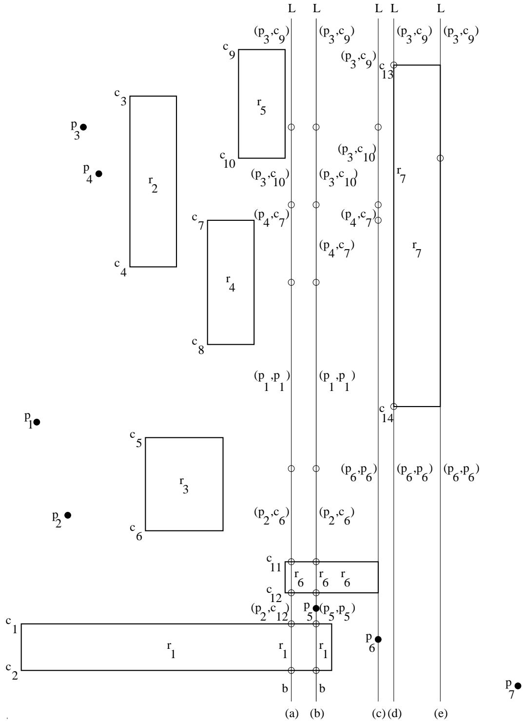
Figure 5: The status of the sweep line is shown at five positions: (a) just before the point event at p_5 , (b) after updating for the point event at p_5 , (c) after updating for the point event at p_6 , (d) after updating for the left event at the left edge of r_7 , and (e) after updating for the right event at the right edge of r_7 . The solid circles are the points p_i of S , the hollow circles are points of the status tree, the r_i are the rectangles, and the c_i are corners on the left edges of rectangles. The labels are shown next to the intervals, and label b = ((-\infty, 0), c_2) .
