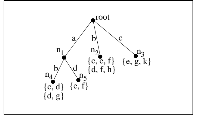
Figure 2: A hash tree \mathcal{T} storing a set of six 4-itemsets X = \{\{a, b, c, d\}, \{a, b, d, g\}, \{a, d, e, f\}, \{b, c, e, f\}, \{b, d, f, h\}, \{c, e, g, k\}\} , where each leaf can store at most two itemsets (only the suffix of an itemset following the prefix defined by the path to the leaf is stored).
